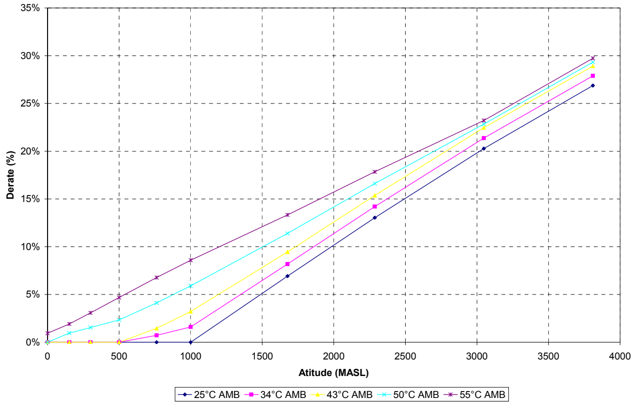
Derate Chart 2206C-E13 TAG3 450 kVA Low E
